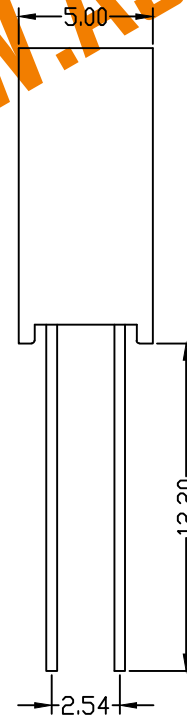
DIP: 12.2 Type1
