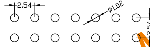
PCB LAYOUT
